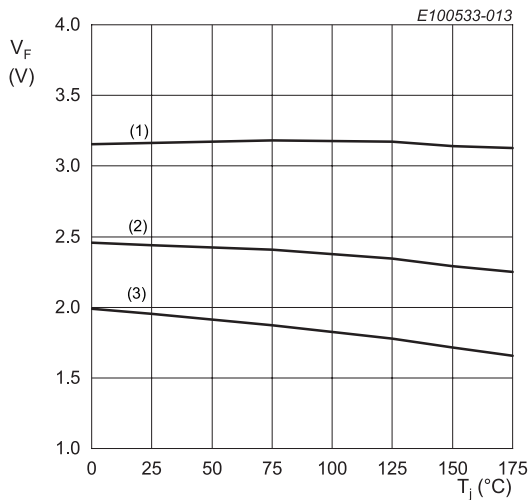
(1) I_F = 30\text{ A} (2) I_F = 15\text{ A} (3) I_F = 7.5\text{ A} Fig. 13. Typical diode forward voltage as a function of junction temperature
