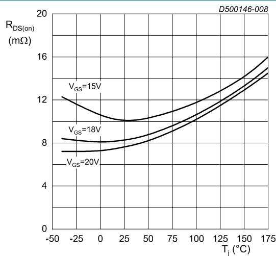
I_{DS} = 100\text{ A}; t_p < 200\text{ }\mu\text{s} Fig. 8. Drain-source on-state resistance as a function of junction temperature
